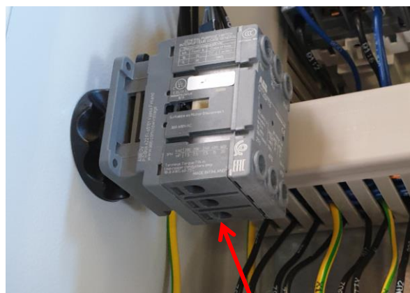
Power connection
