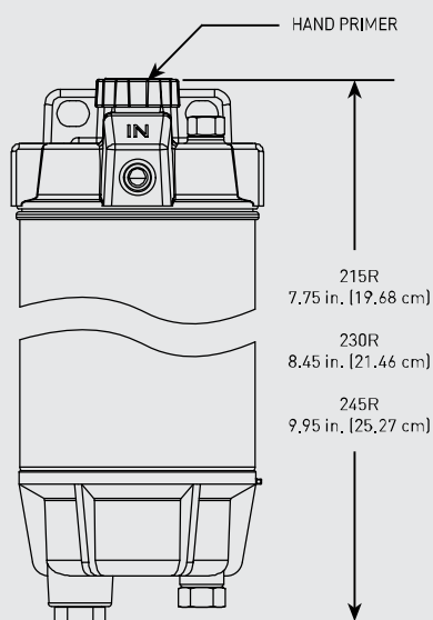
200 Series Front
