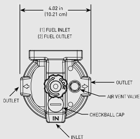
200 Series Top
